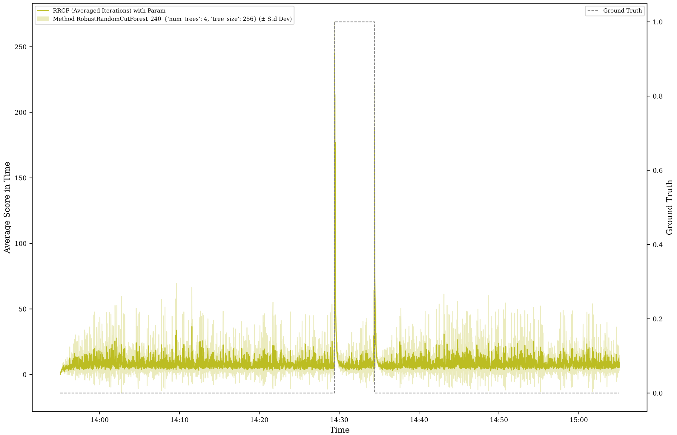
Method RRCF Score for Scenario A2
